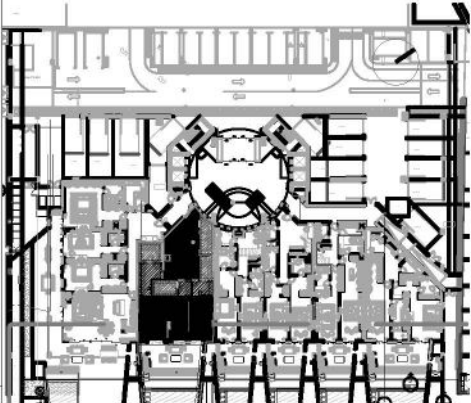
BLOCK PLAN
